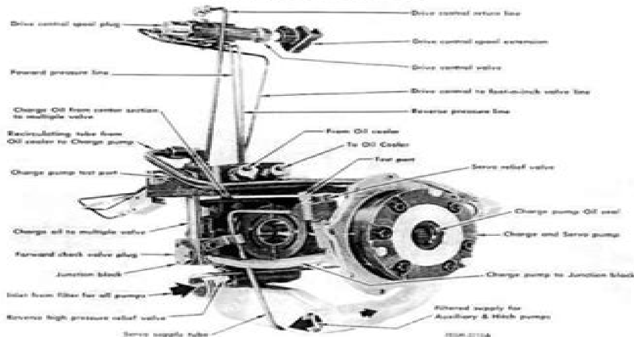
Illustr. 7. Hydraulic components (front view) less hydrostatic pump, motor, swash plates and servos.
