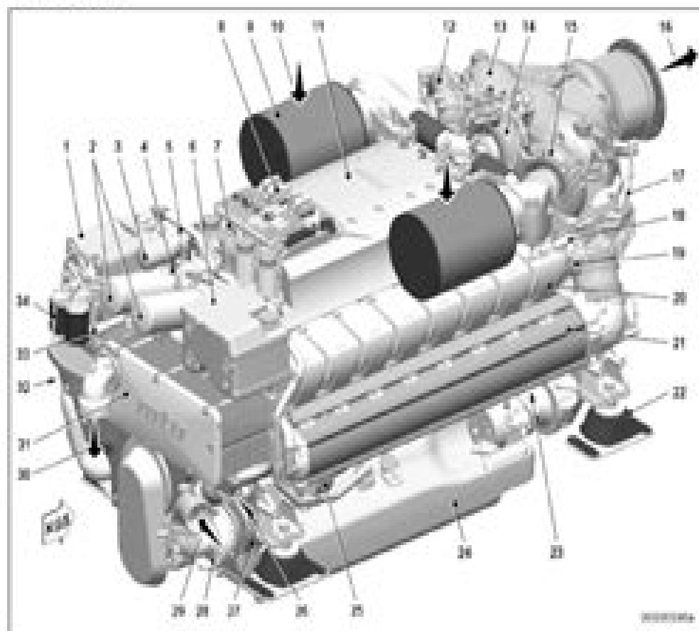
Engine layout
