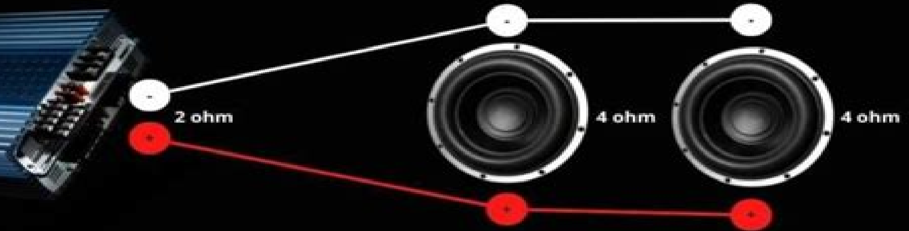
Two SVC 4 ohm subs in parallel with single amp's channel
