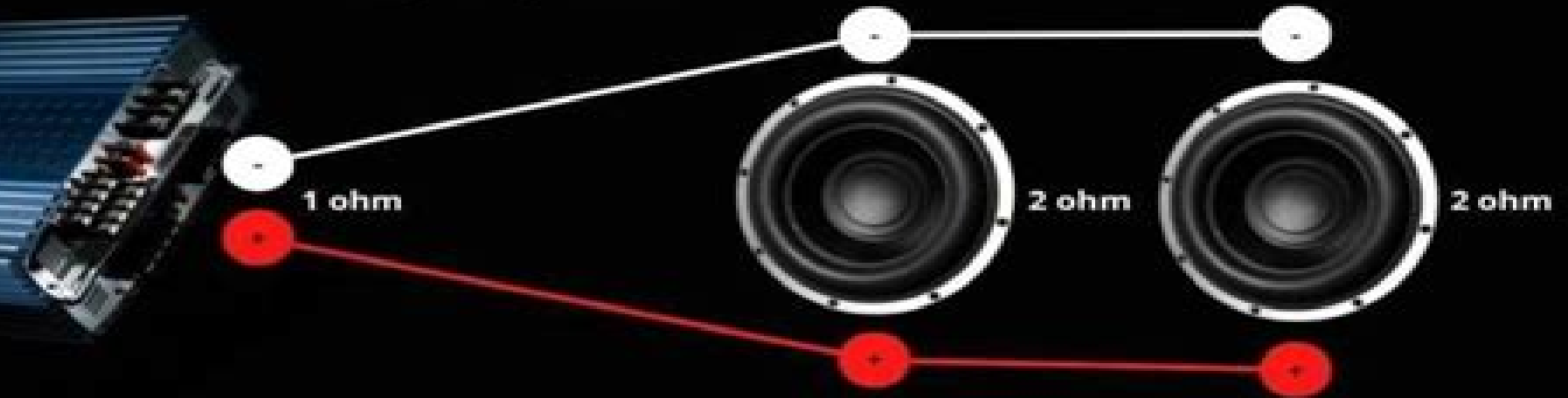
Two SVC 2 ohm subs in parallel with single amp's channel
