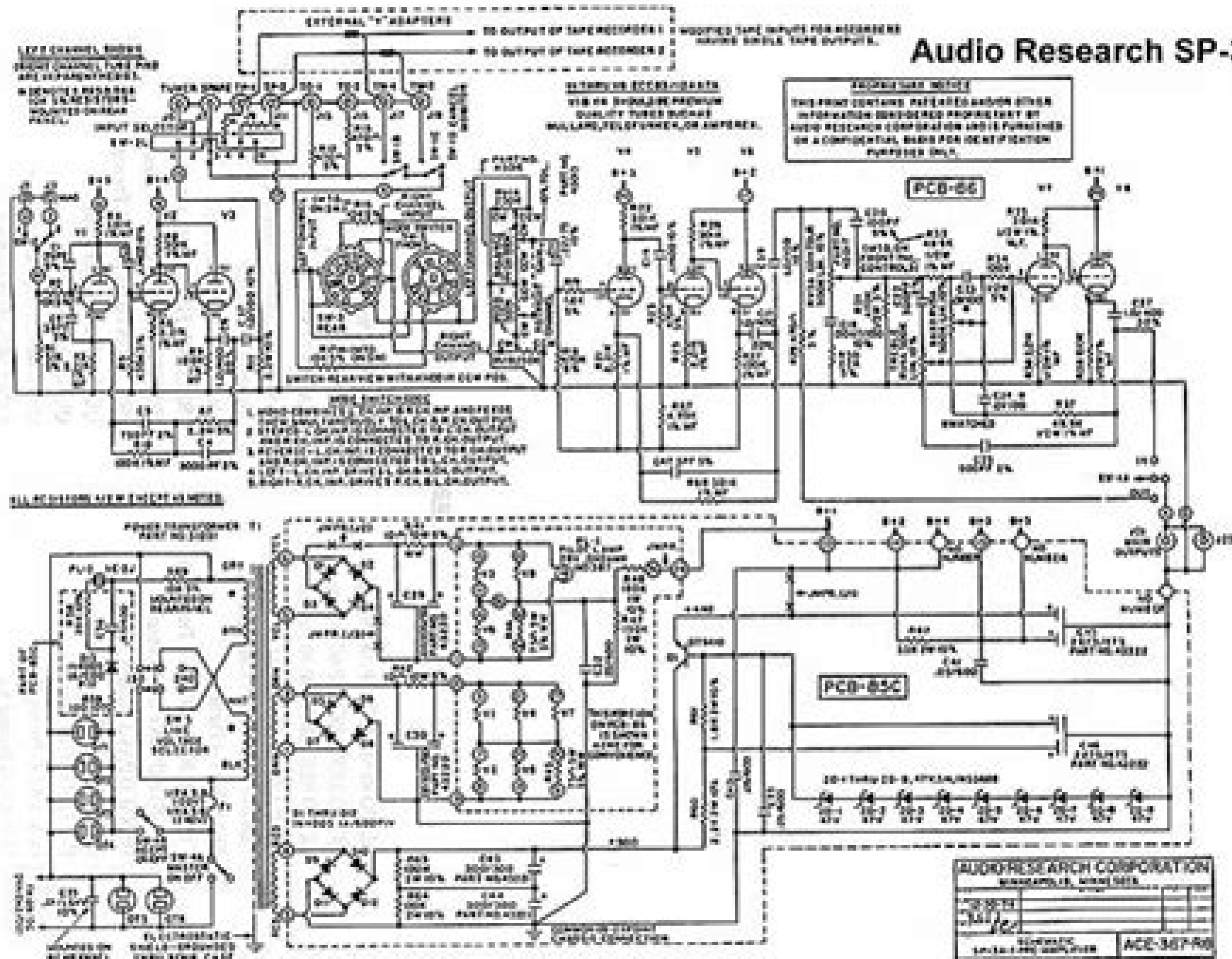
SCHEMATIC DIAGRAM
