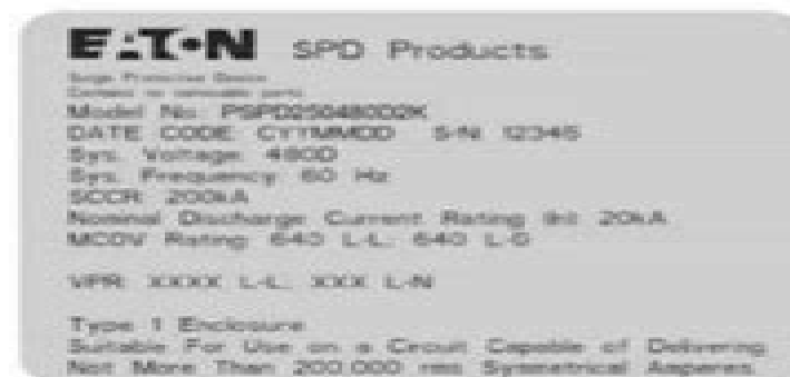
Figure 1. Product Label
