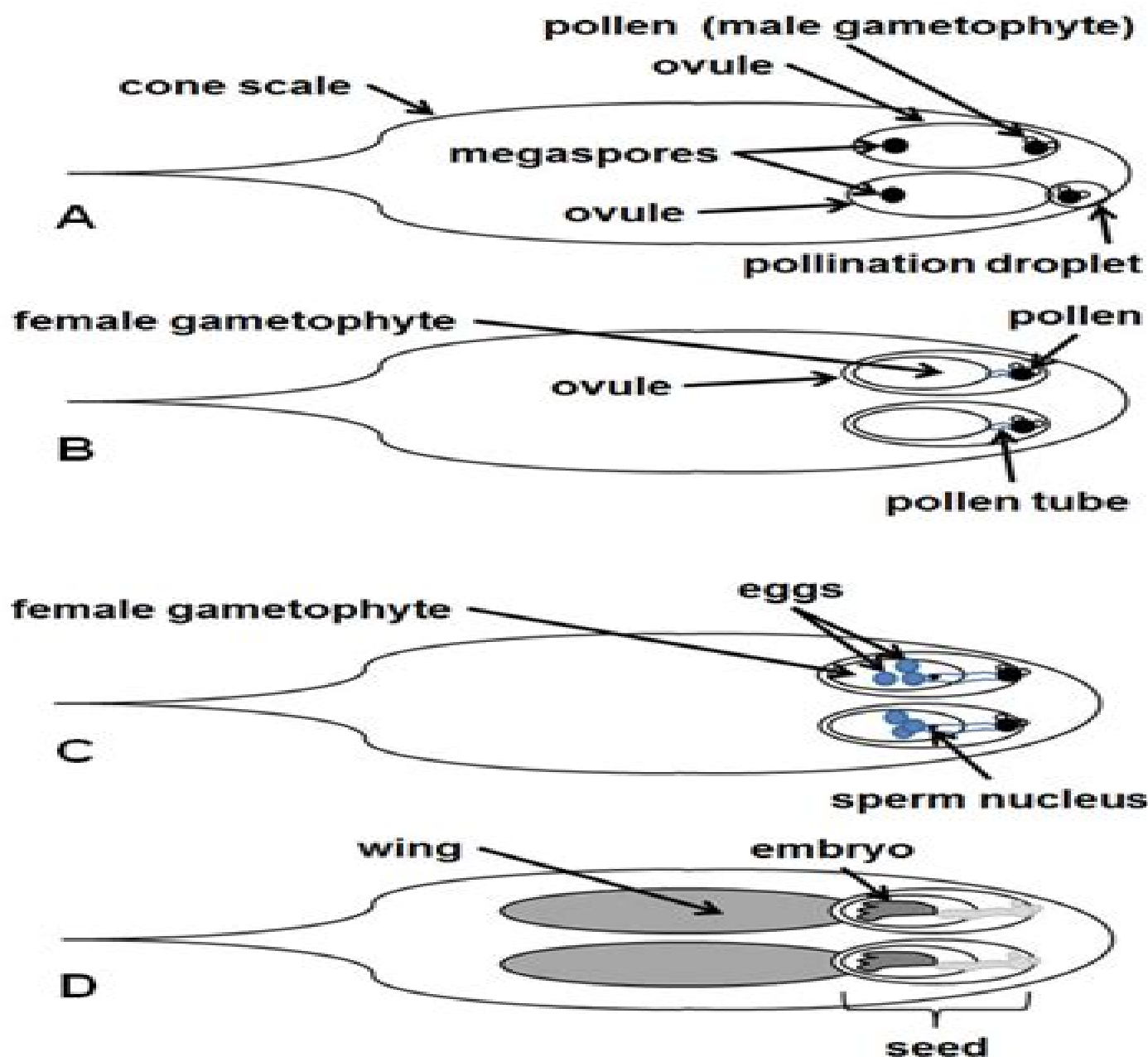
Fig. 13. Development in cone scales in Pinus virginiana .
