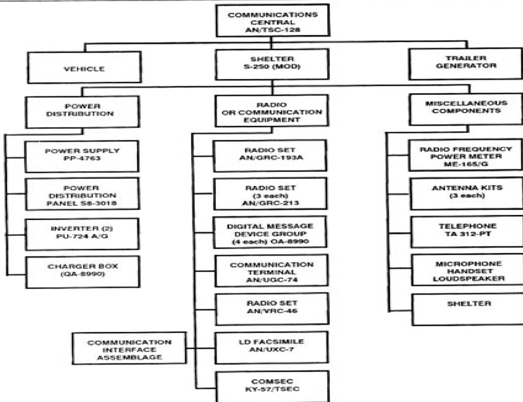
Figure D-16. Composition of AN/TSC-128.
