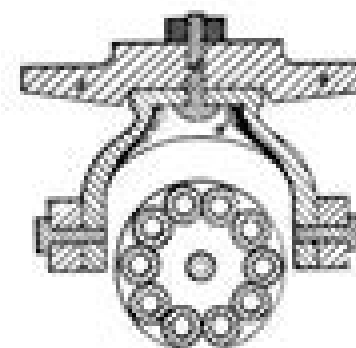
FIG. 5. SECTION THROUGH TRUNNION PLATE, TRUNNIONS AND PIVOT BLOCK.
