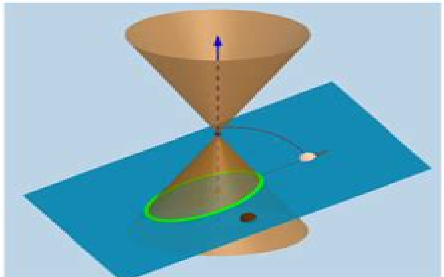
Ellipse
