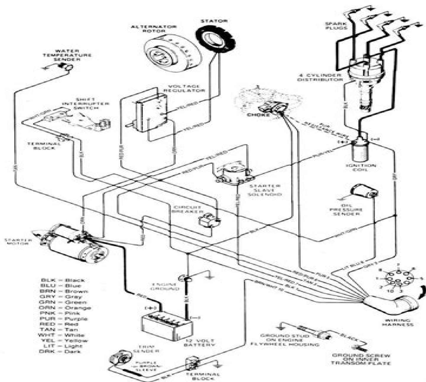
Engine Electrical System Wiring Diagram
