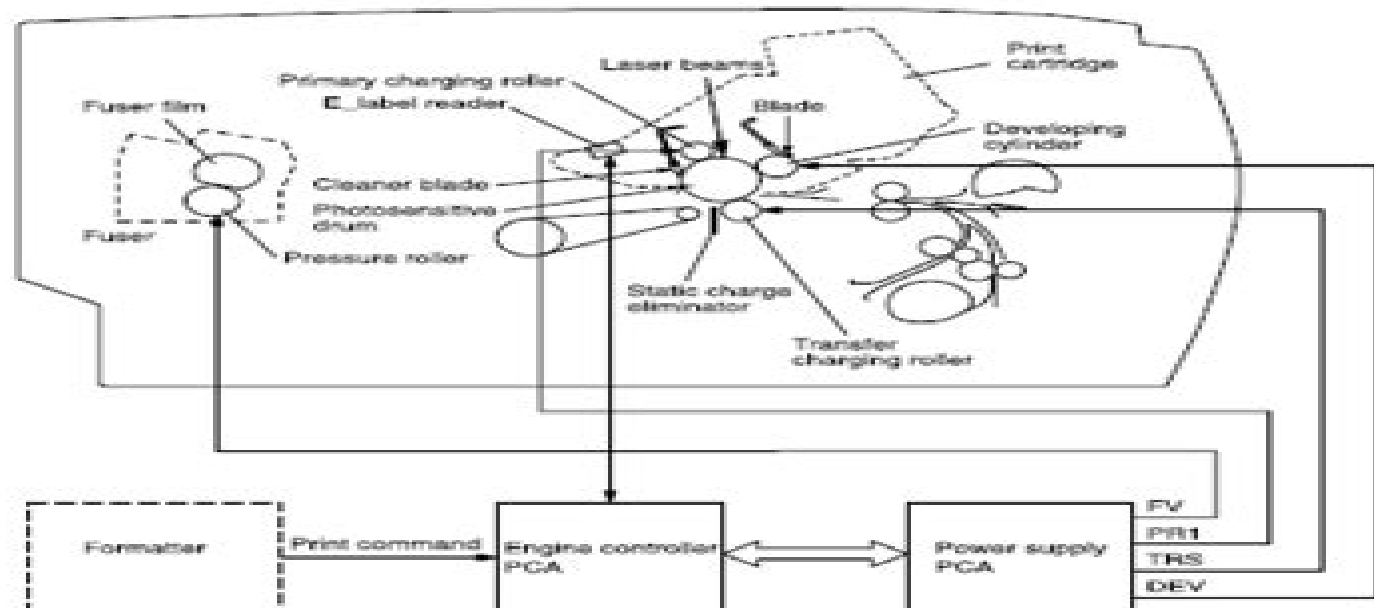
Figure 18. Image-formation system
