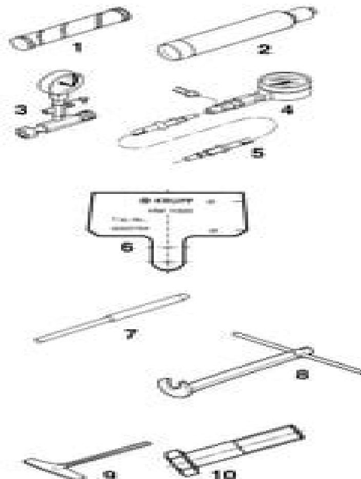
Fig. 2 Service tools
