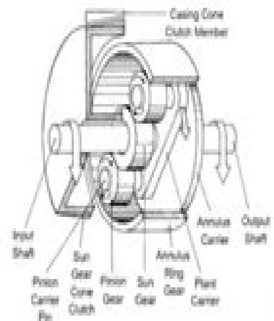
Epicyclic Gearbox
