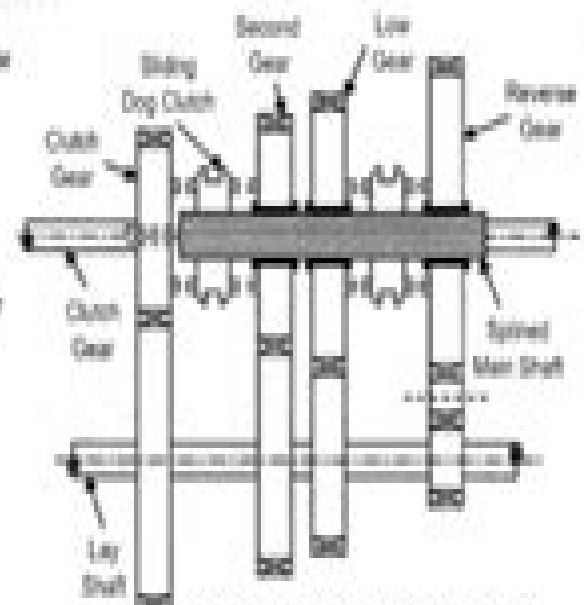
Constant Mesh Gearbox
