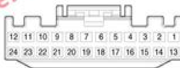
A Connector [B01-1A] (24pin)
