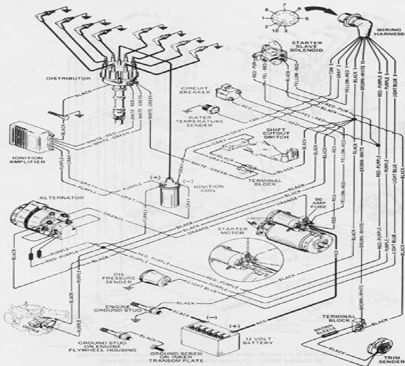
MCM 200 5.0 Litre Engine with 90 Amp Fuse at Starter Motor (Orange Wire) (Battery Meter Circuit)
