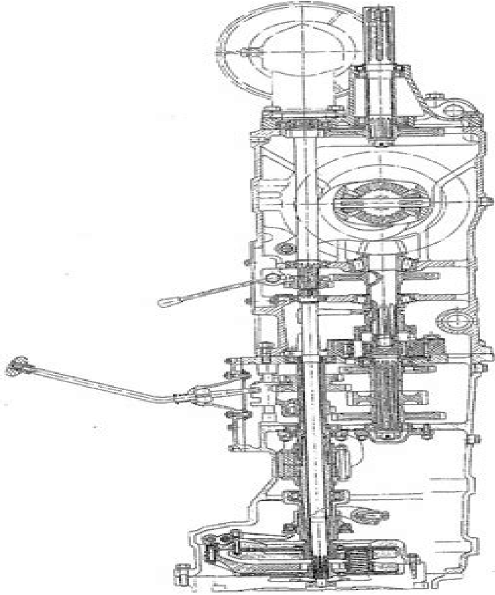
Fig. 11. - Transmission longitudinal section.
