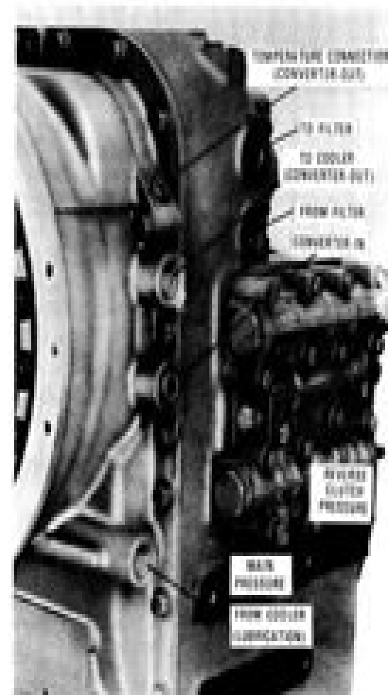
FIG. 10 PRESSURE AND TEMPERATURE CHECK POINTS
