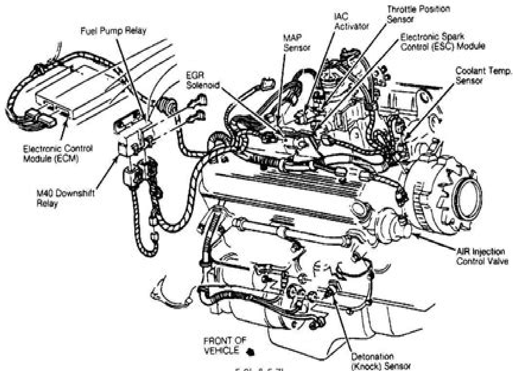
Fig. 4: Component Locations (4 Of 11)
