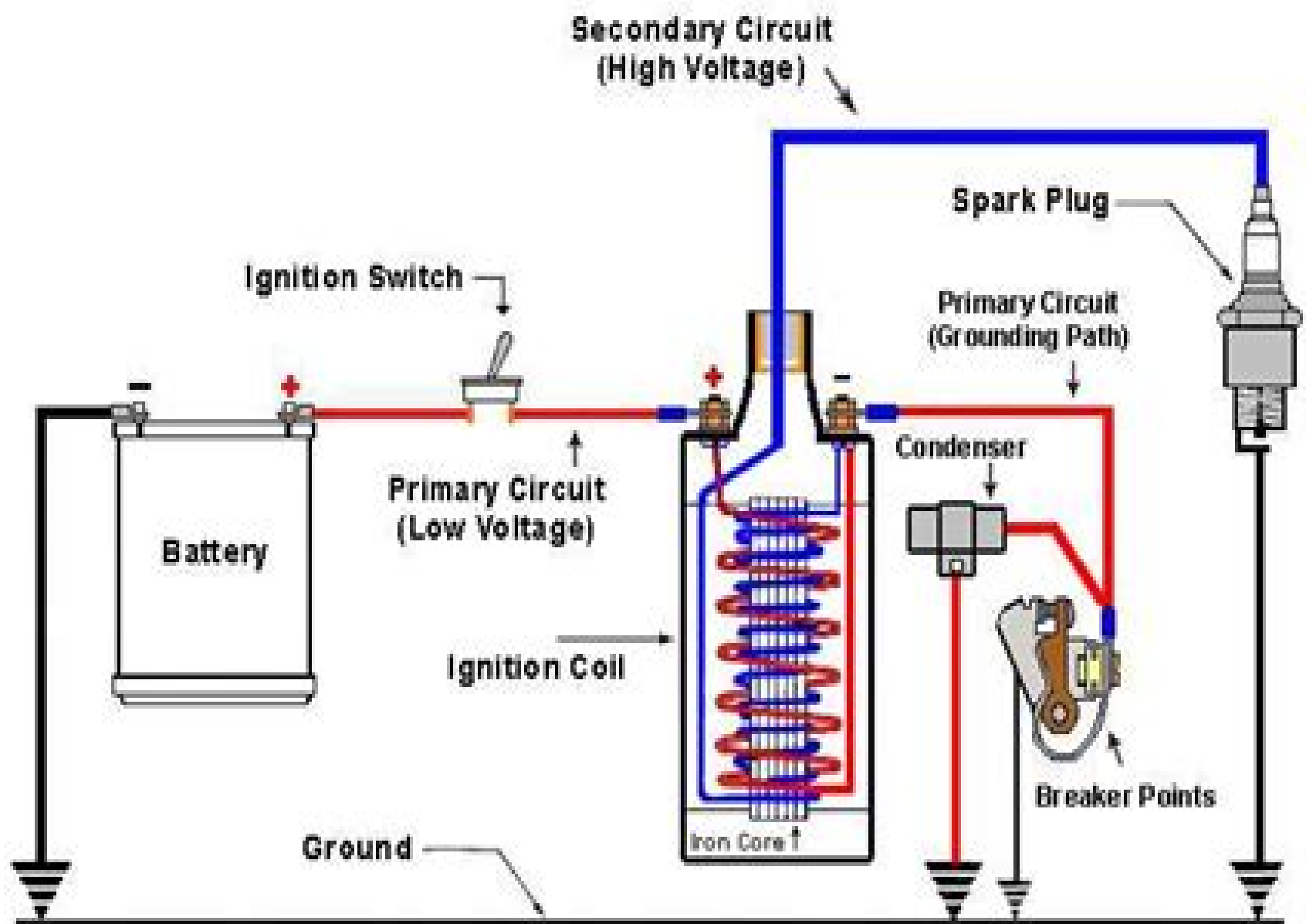
Primary (red) and Secondary (blue) Ignition Systems
