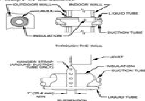
Fig. 1 – Piping Installation
