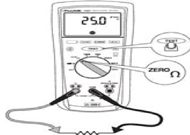
Measuring Earth-Bond Resistance
