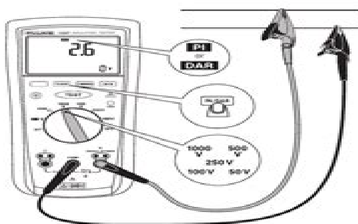
Polarization Index and Dielectric Absorption Ratio (1507)
