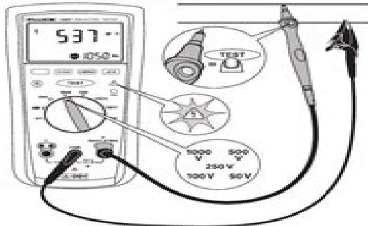
Measuring Insulation Resistance
