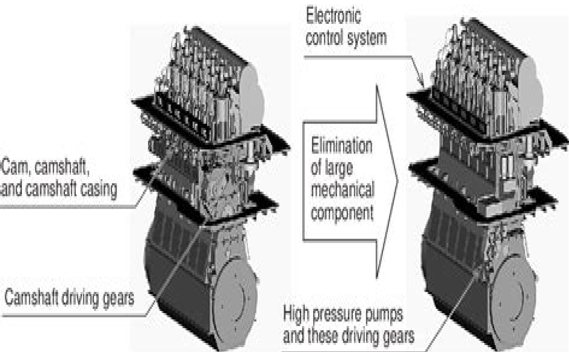
Fig. 1 Fundamental structure of engine
