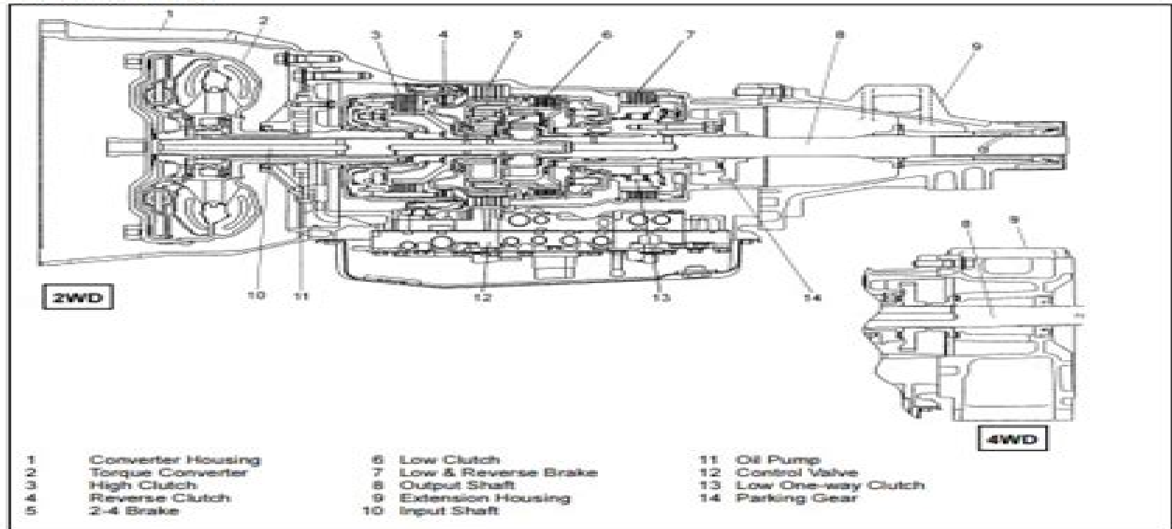
Figure 1. Construction of Automatic Transmission
