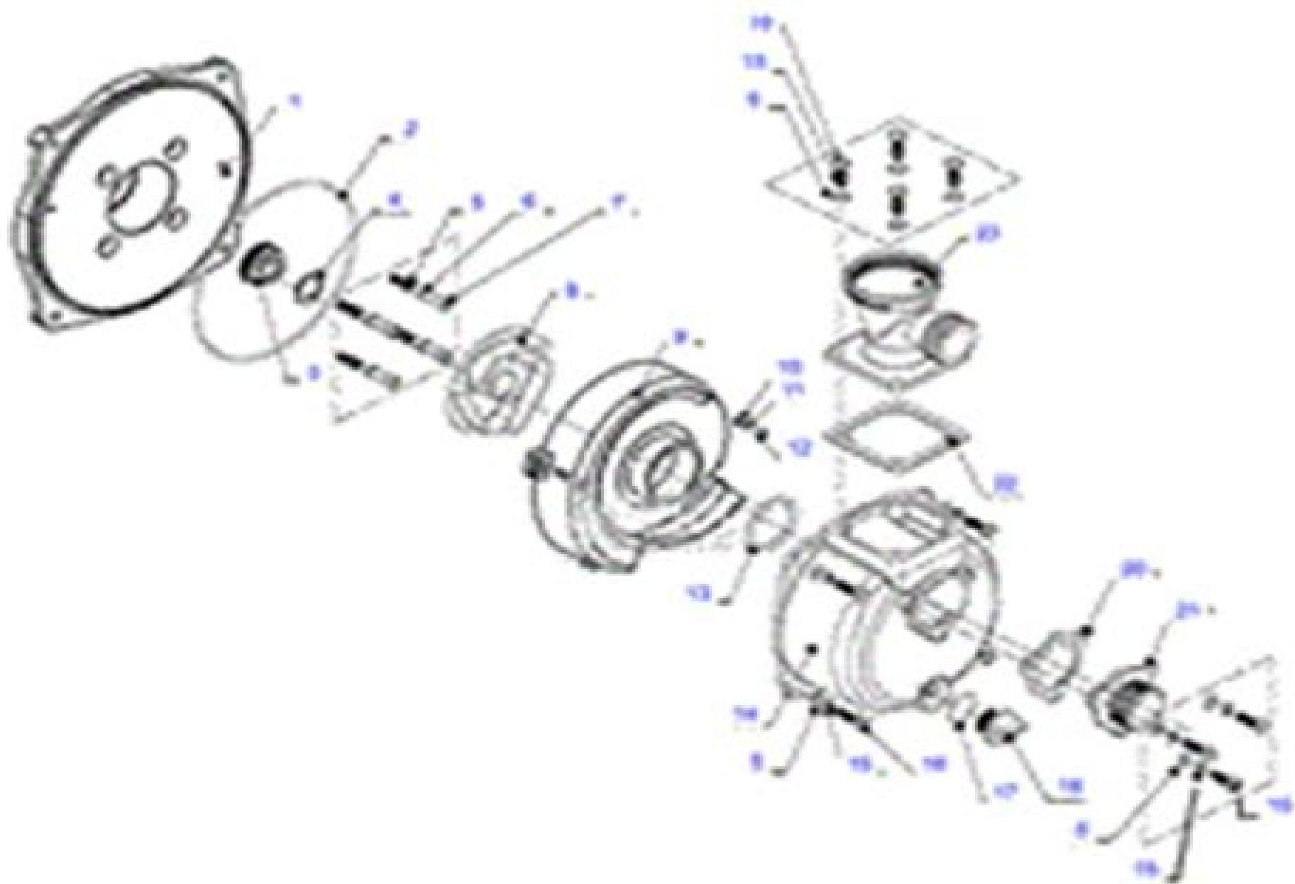
Exploded view of the pump assembly
