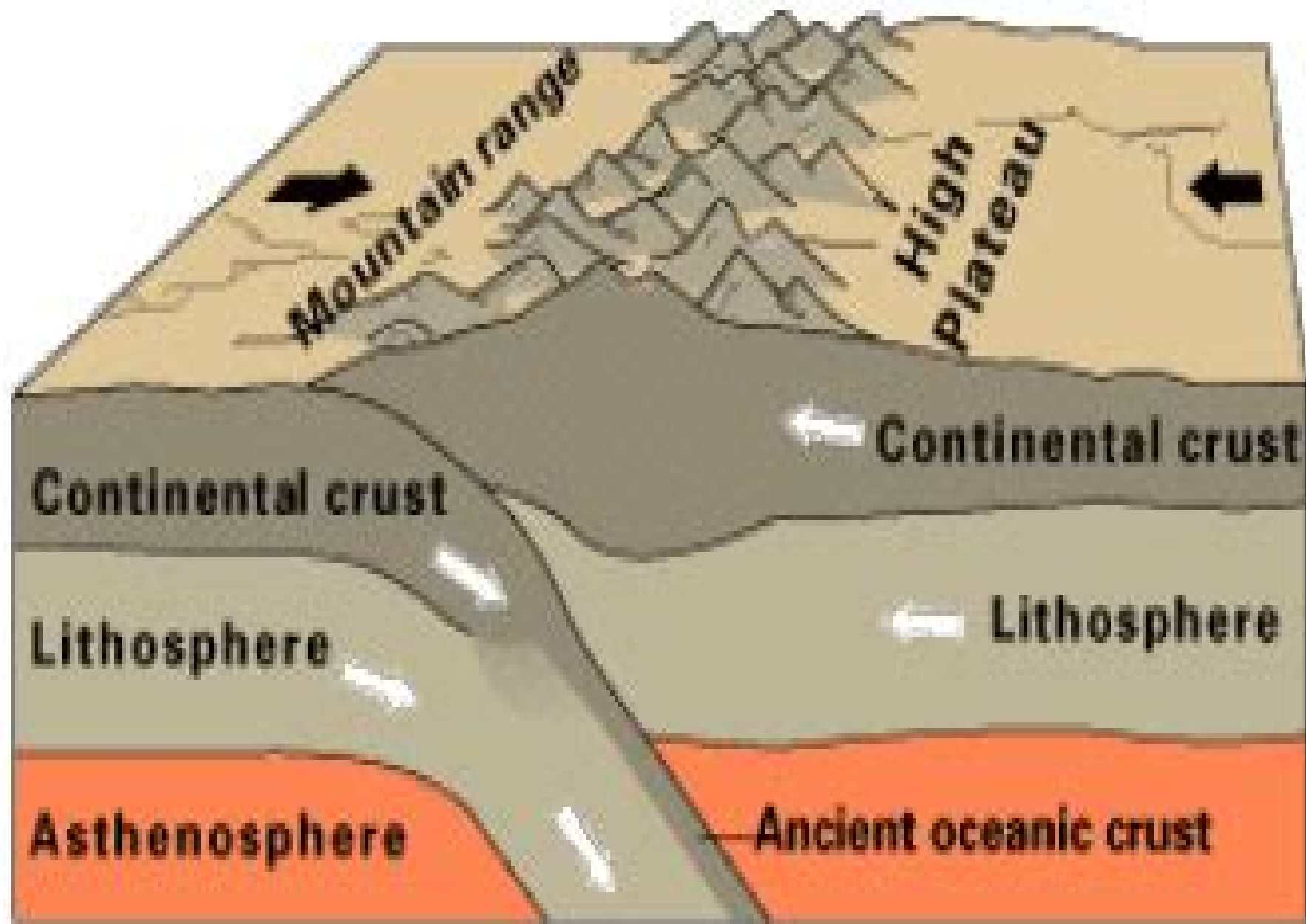
Continental-continental convergence
