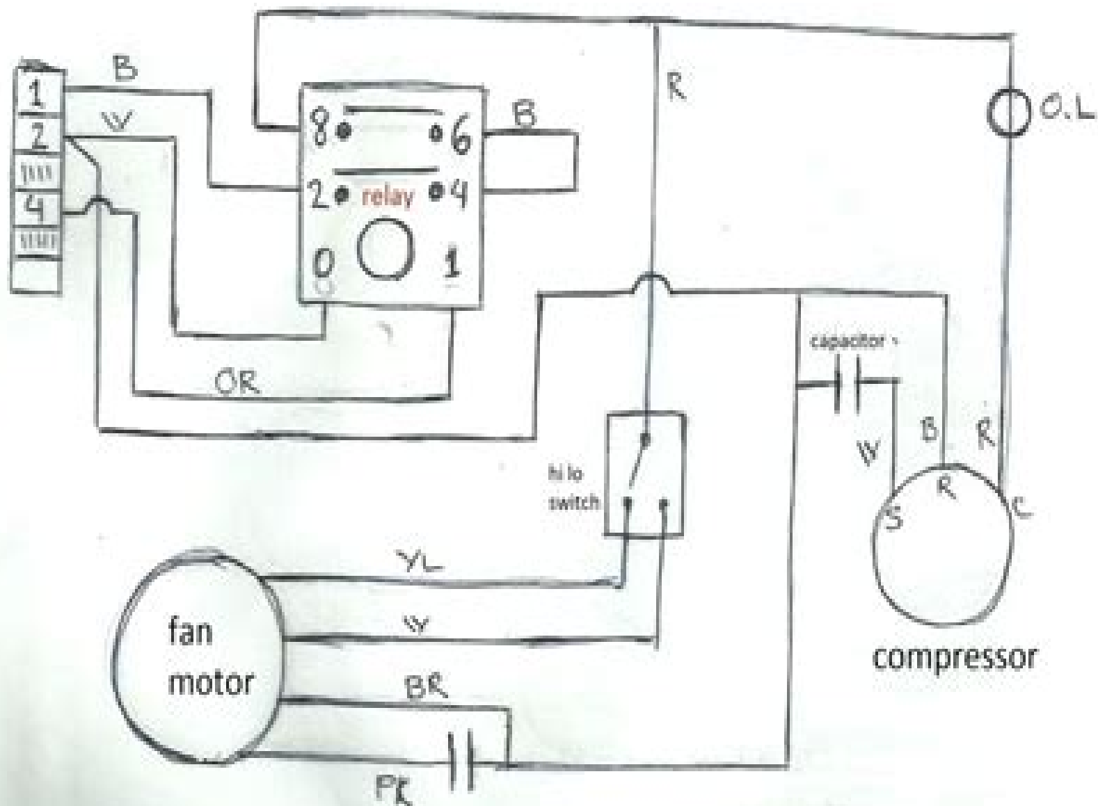
Outdoor Unit
