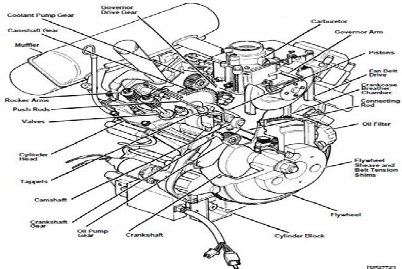
Cutaway—FD620D
