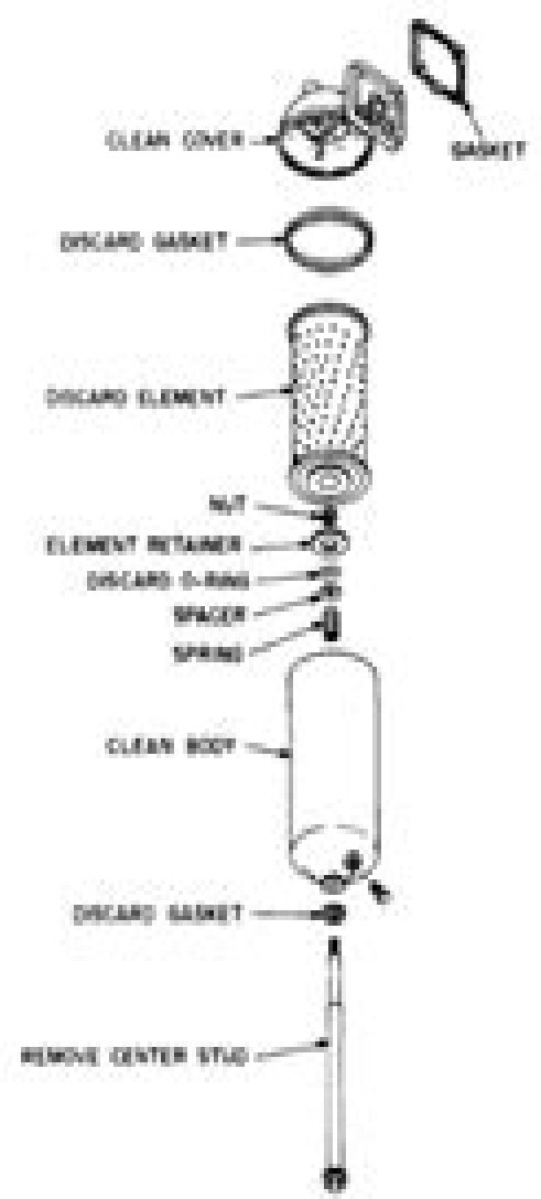
Figure 4-2. Oil filter service.
