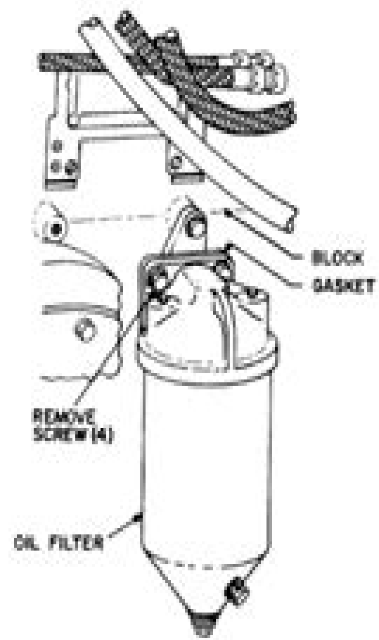
Figure 4-1. Oil filter, removal and installation.
