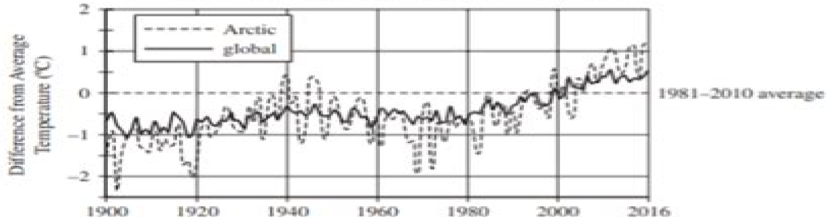
CHANGES IN AVERAGE TEMPERATURE, 1900–2016
