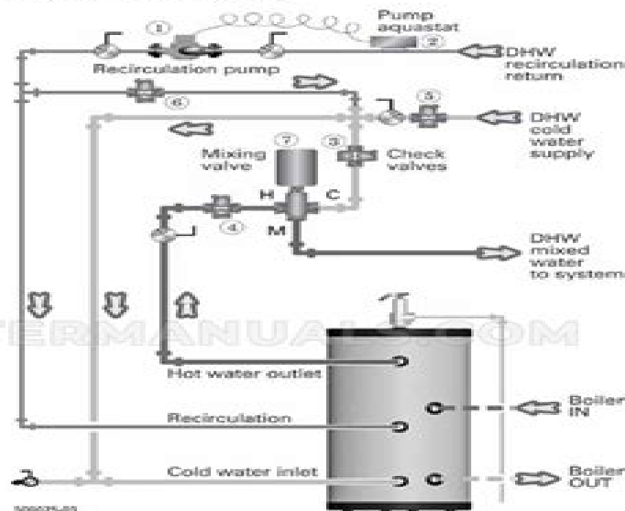
Figure 6 Recirculation piping
