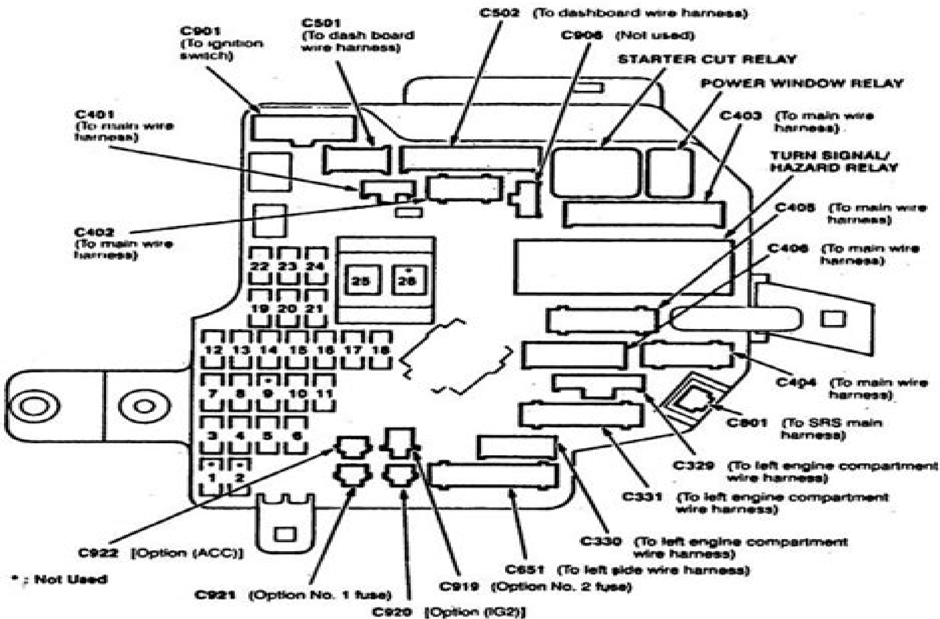
I/P Fuse/Relay Box
