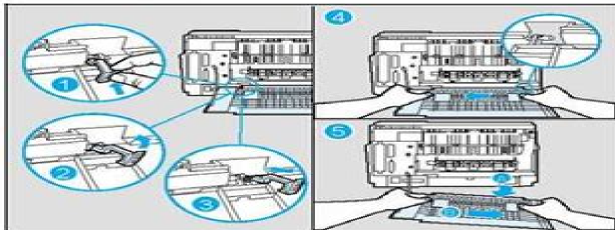
Figure 6-7b Releasing the Door Hinge (LaserJet 4 Plus)
