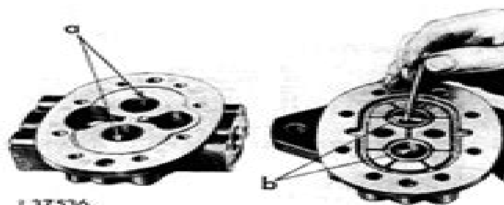
Fig. 3 — Checking Position of Oil Grooves and Dimension of Bushing Bores
