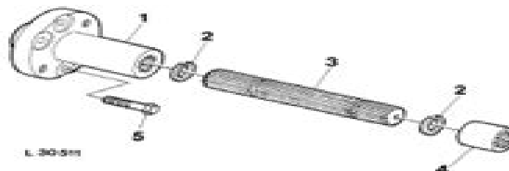
Fig. 4 — Pump Drive, Exploded View
