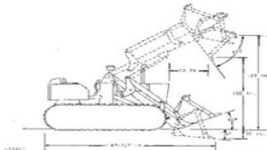
JCN50-B Loading Dimensions
