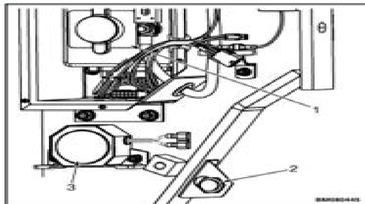
Figure 18. Lift Proximity Sensor Location
