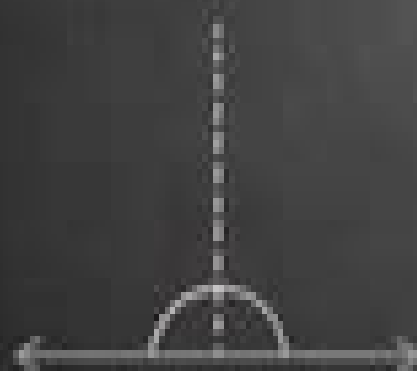
straight angle
