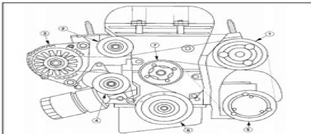
11.11B Auxiliary drivebelt routing
