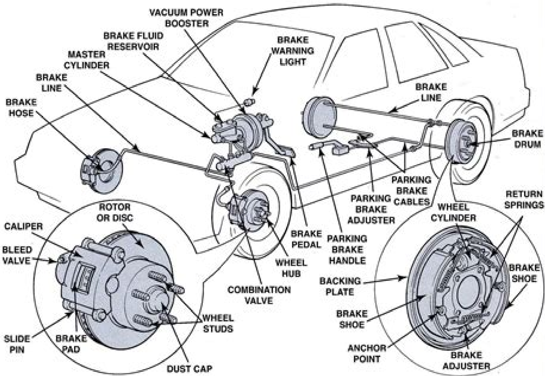
DISC BRAKE
