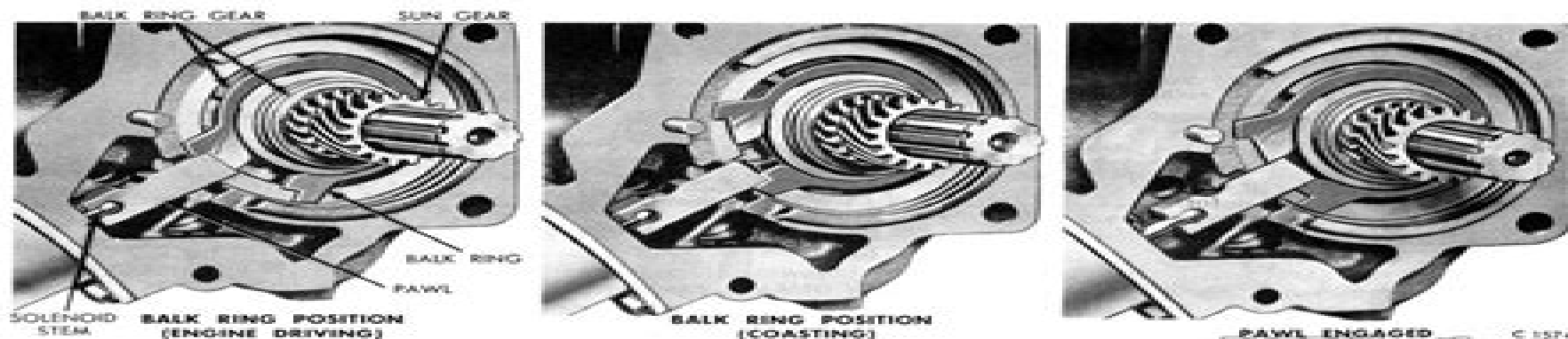
FIG. 8—Balk Ring and Pawl Operation
