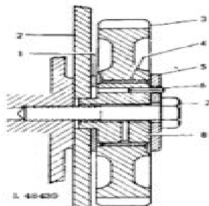
Fig. 5 -- Upper Idler Gear Installed, Sectional View
