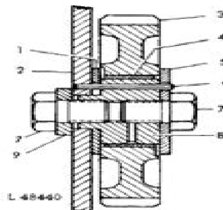
Fig. 6 -- Lower Idler Gear Installed, Sectional View
