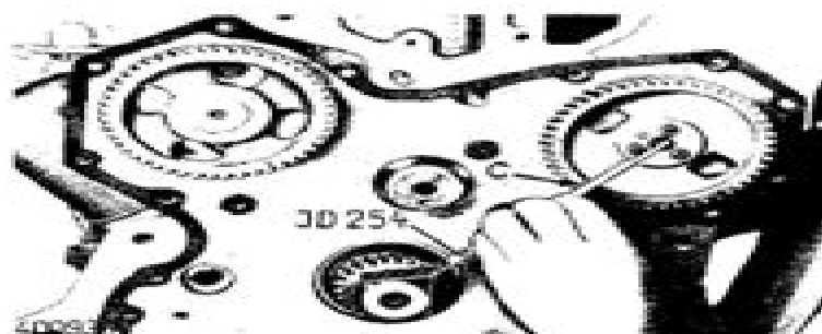
Fig. 4 -- Timing Injection Pump Gear, Using Timing Tool No. JD 254
