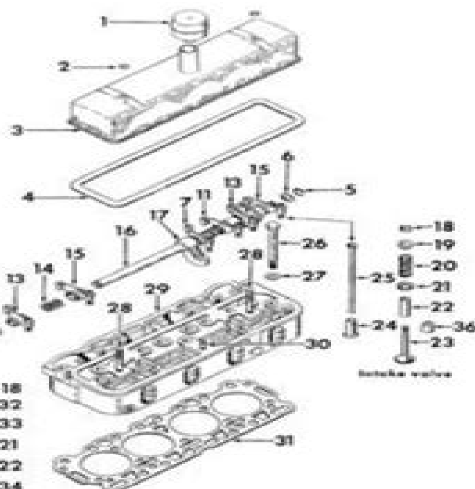
Intake valve
