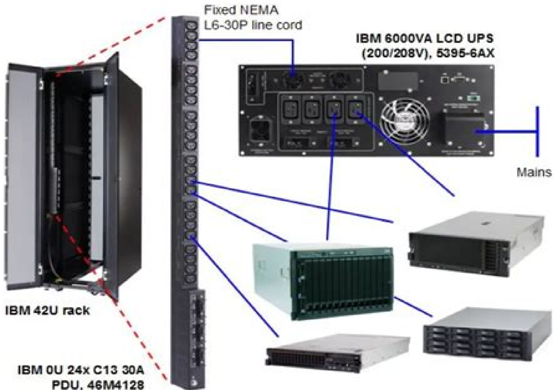
Figure 5. Sample configuration showing use of the 6000VA LCD 4U Rack UPS (200/208V) with a PDU
