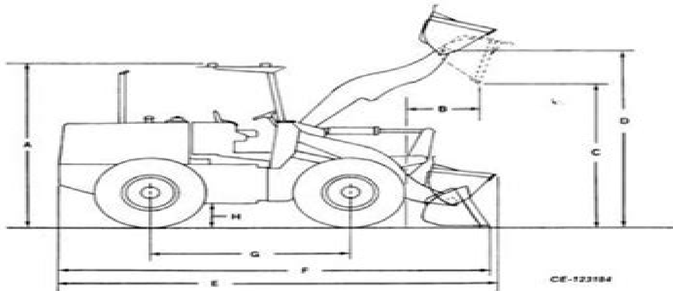
FIG. 1 — General Dimensions
