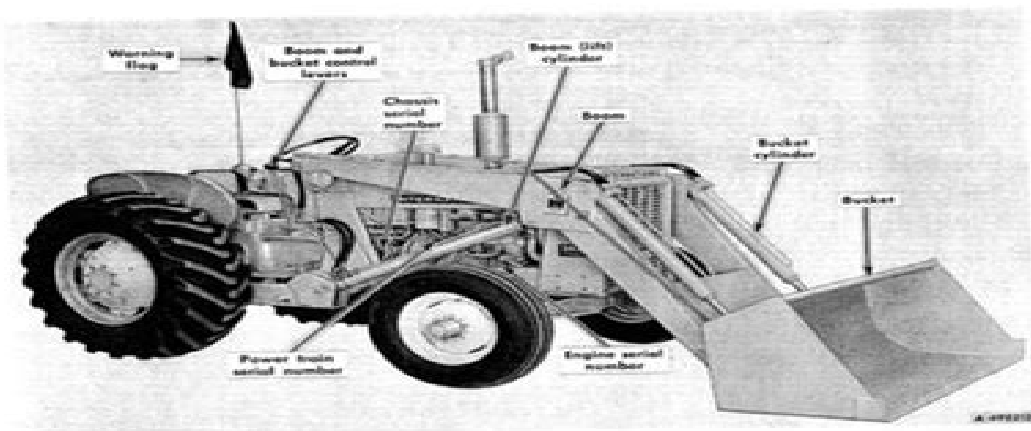
Right Front View of the International 3414 Loader Tractor
