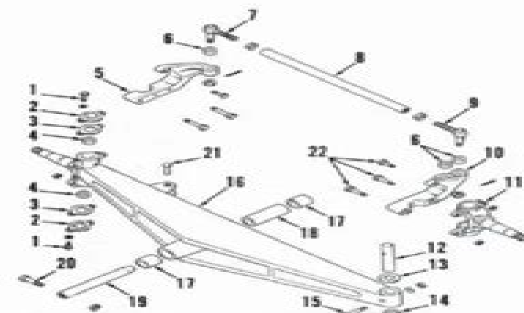
Fig. 6—Exploded view of heavy duty (cast) nonadjustable front axle used on some tractors.
