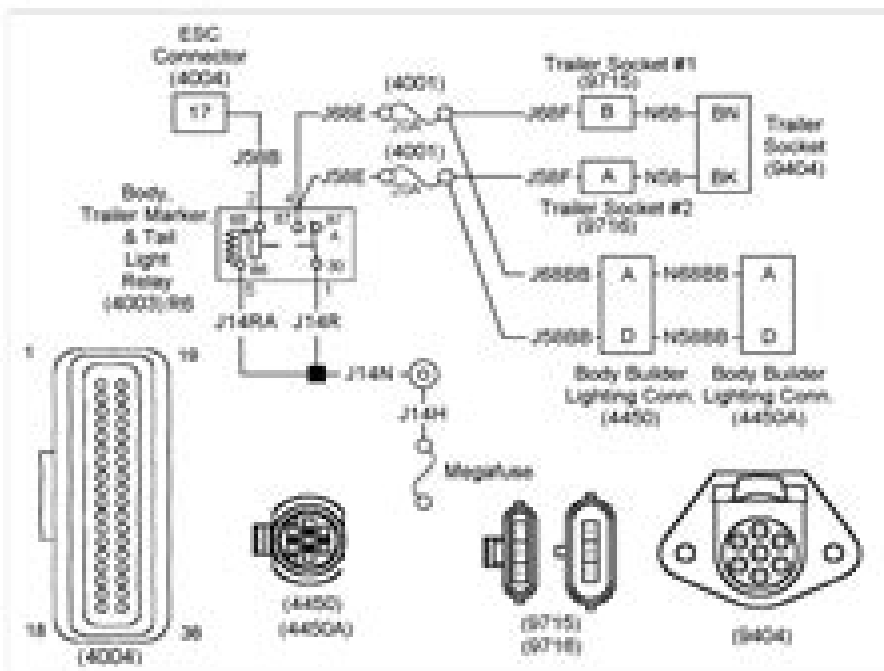
Figure 3-48 Body, Trailer Marker & Tail Light Relay Circuits—Always Refer To Circuit Diagram Book For Latest Circuit Information
