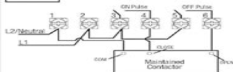
ET1725-Pulse 2x SPST
