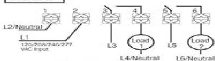
ET1725-2x SPST
