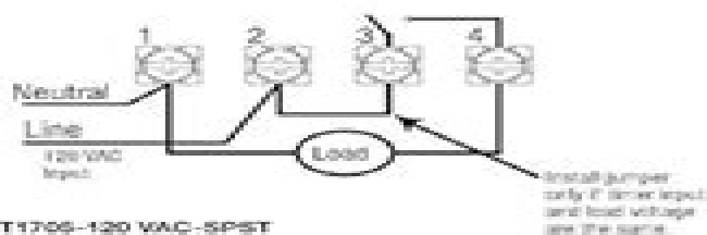
ET1705-120 VAC-SPST
