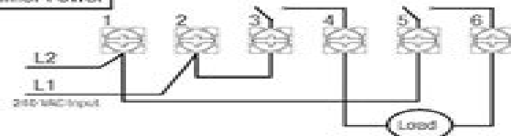
Timer Power
