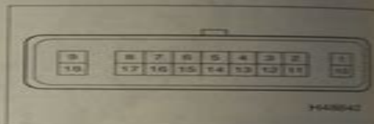
18.4d ABS control unit wiring connector terminal numbering - loom side
