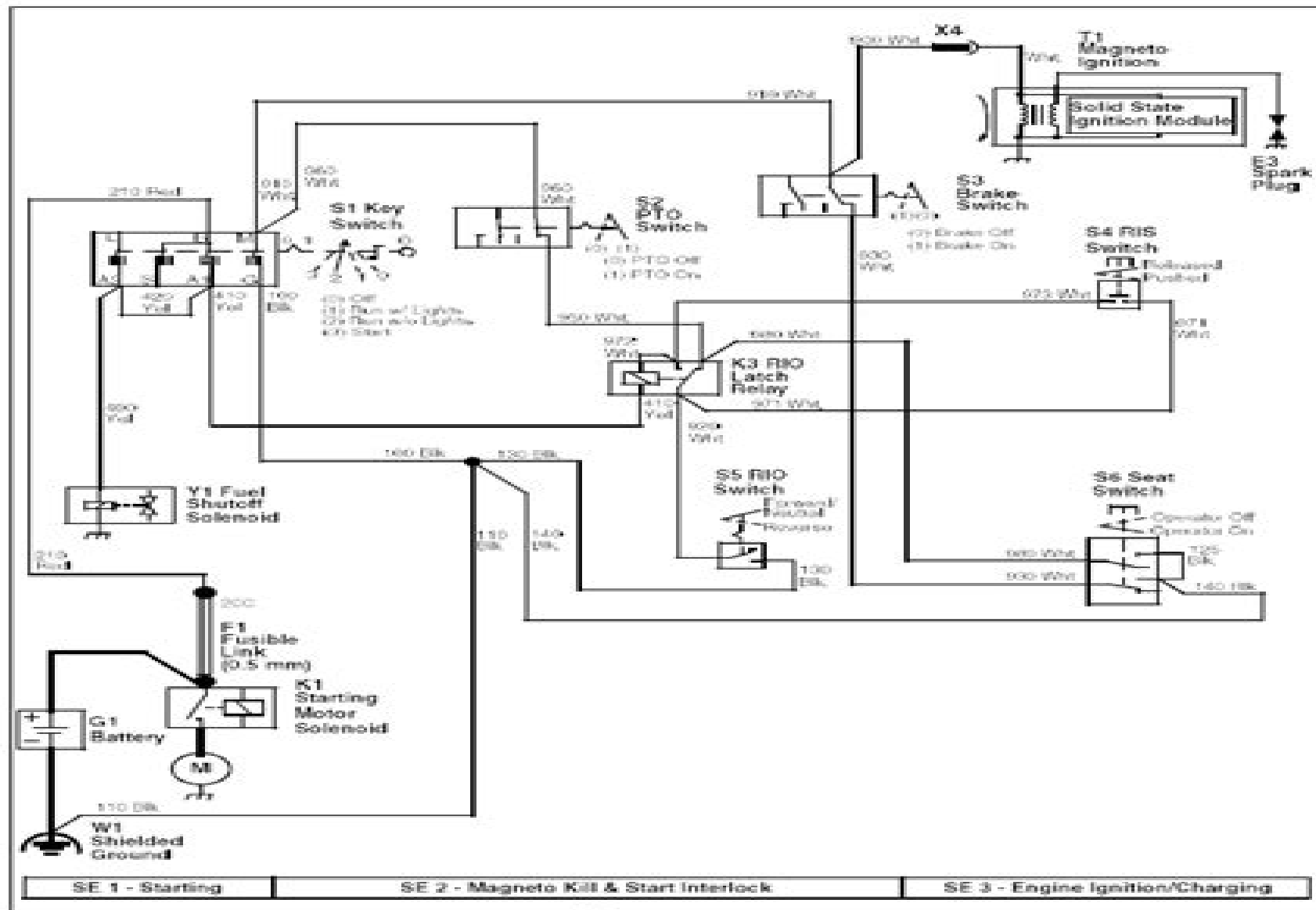
PTO with RIO Circuit Schematic - LT150 and LT160
