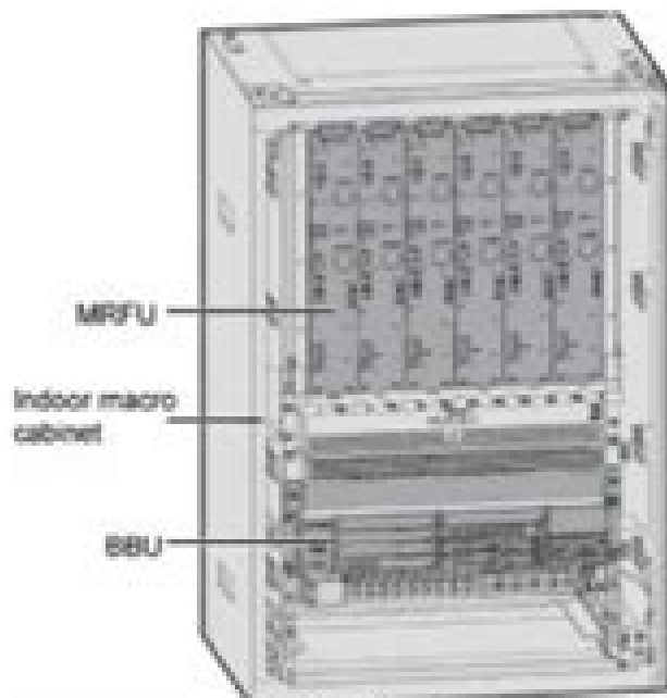
BTS3900 system structure
